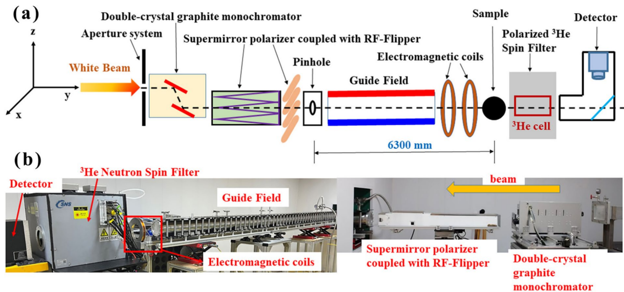
Fig. 1 (Color online) a Schematic illustration of PNI setup at the beamline CNGC at the CARR. b Physical picture of the designed PNI setup
