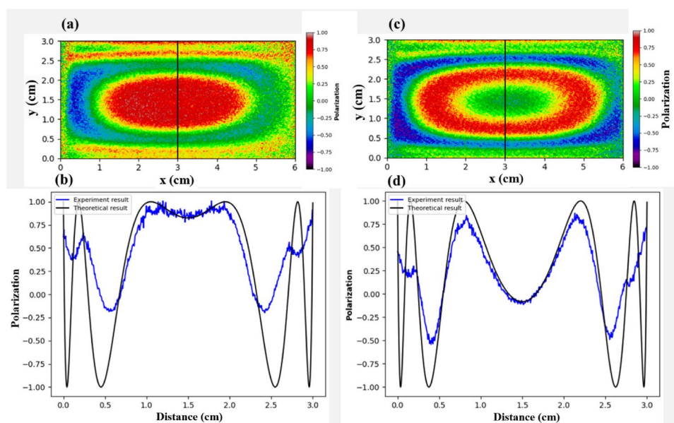
Fig. 7 (Color online) Comparison between experimental and initial theoretical fitting results for the tested solenoid
