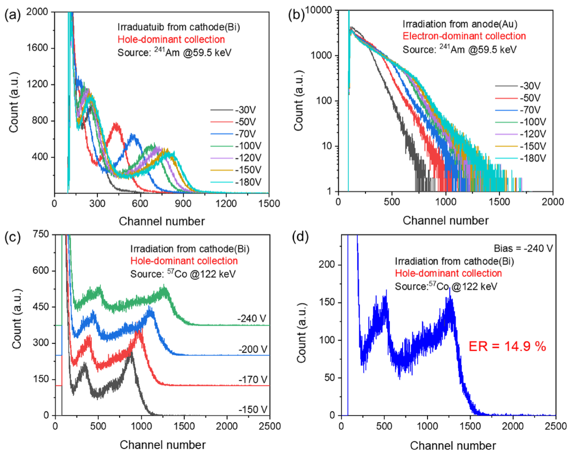
Fig. 5 (Color online) \gamma -ray response by the Schottky-type CsPbCl 3 detector under a hole dominant transport and b electron dominant transport collection under ^{241}\text{Am} \gamma -rays. c ^{57}\text{Co} \gamma -ray spectrum by
