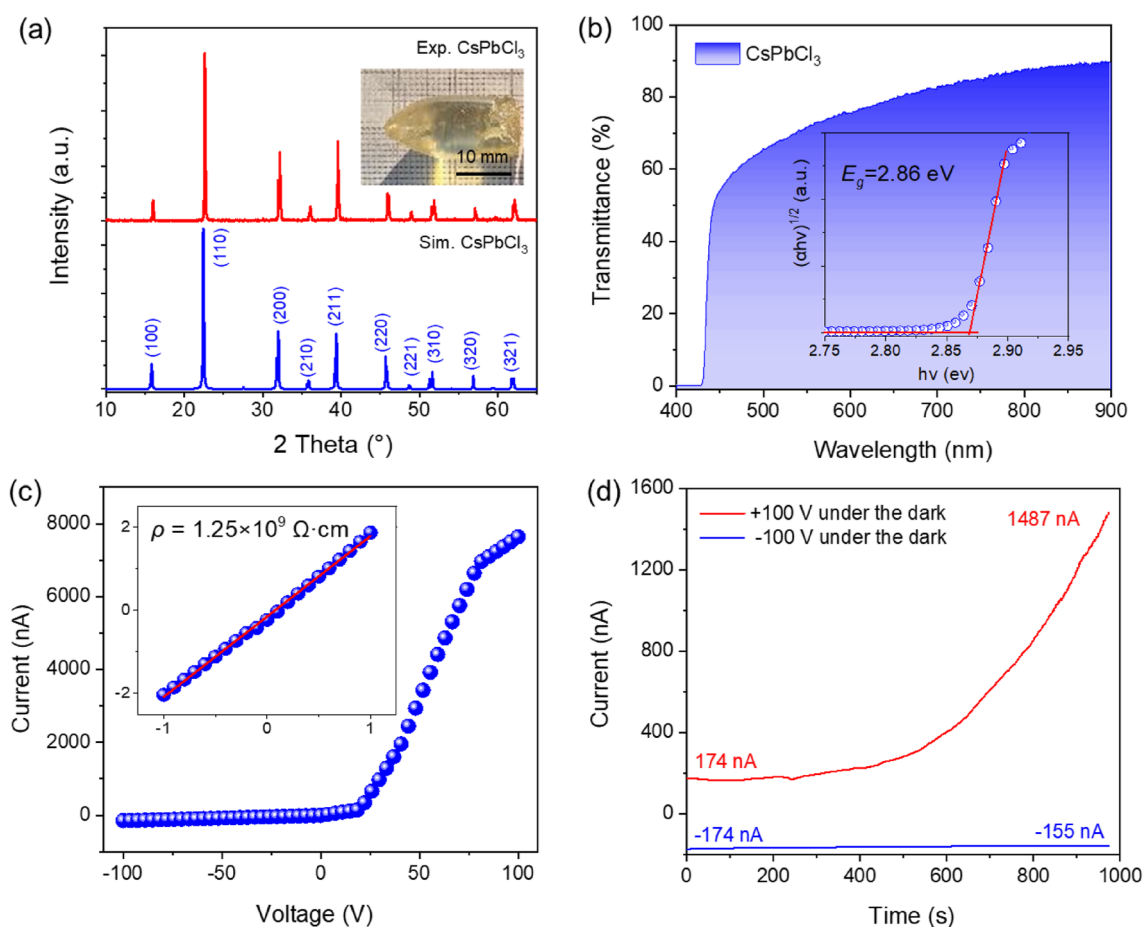
Fig. 1 (Color online) a Powder XRD patterns of the \text{CsPbCl}_3 crystal. The inset corresponds to the \text{CsPbCl}_3 ingot. b Transmission spectra for the \text{CsPbCl}_3 single crystal. Inset: Tauc plot showing the direct bandgap of 2.86 eV. c Typical I - V characteristic curve of a Schottky-
