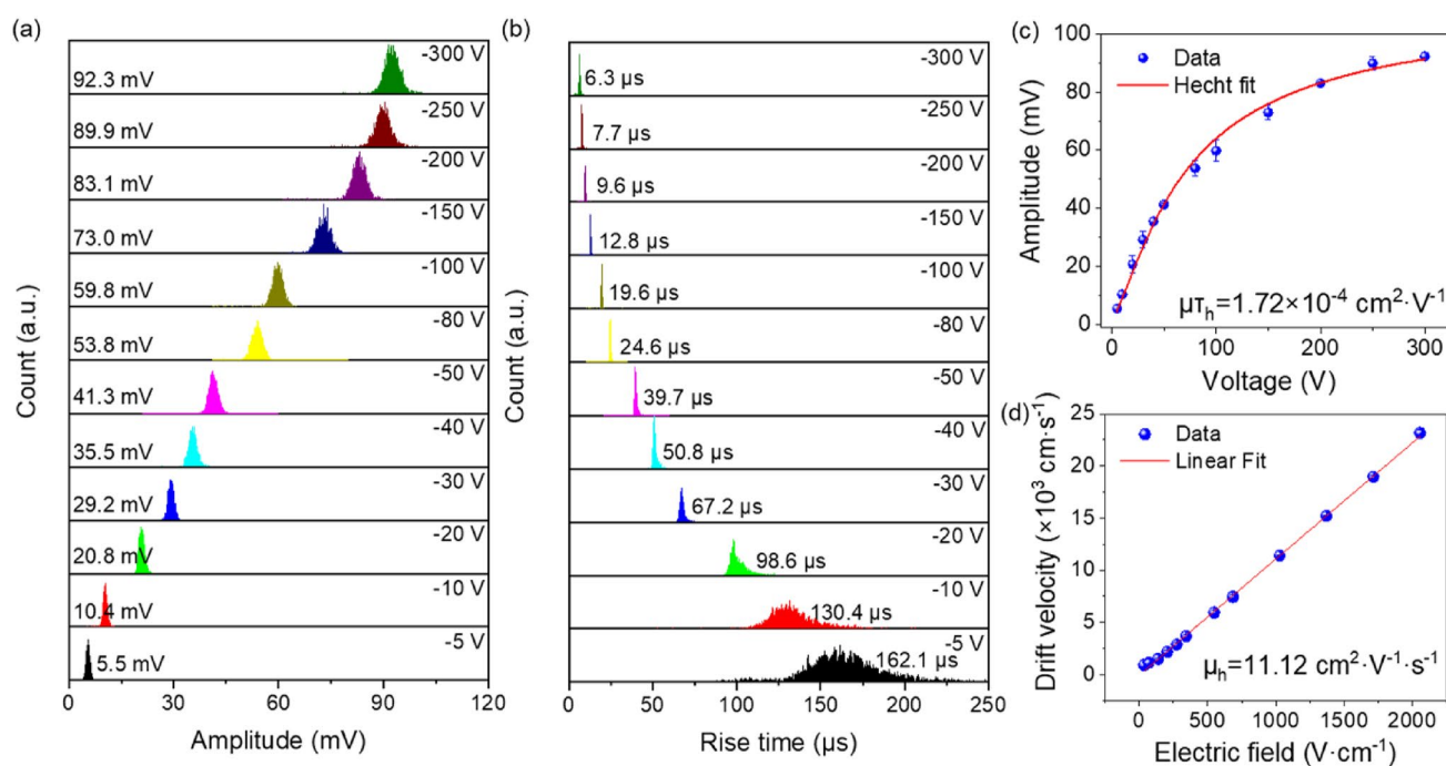
Fig. 4 (Color online) a Amplitude distribution (2000 events) attributed to hole drift based on the transient pulse analysis for ^{241}\text{Am} \alpha particles. b Rise time distribution (2000 events) attributed to hole
