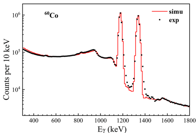
Fig. 2 (Color online) Geant4 simulation for ^{60}\text{Co} \gamma source
