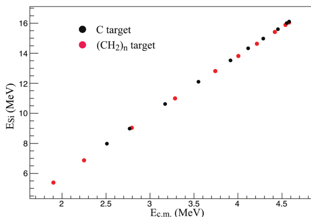
Fig. 5 (Color online) Relationship between E_{\text{c.m.}} and the deposited energy in silicon for the p_1 exit channel
