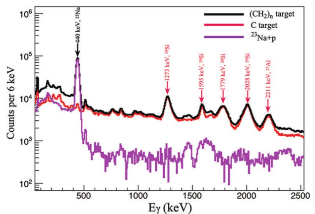
Fig. 4 (Color online) \gamma ray single-energy spectrum measured with the LaBr 3 detector array in coincidence with protons. The \gamma spectrum obtained with (\text{CH}_2)_n target and carbon target is presented as black and red lines, respectively. The purple line is the net count spectrum obtained by subtracting the carbon background spectrum after beam normalization
