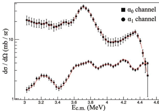
Fig. 9 (Color online) Excitation function for the \alpha exit channels. \alpha_0 and \alpha_1 represent ^1\text{H}(^{23}\text{Na}, \alpha_0)^{20}\text{Ne} and ^1\text{H}(^{23}\text{Na}, \alpha_1)^{20}\text{Ne}^*_{1634} , respectively
