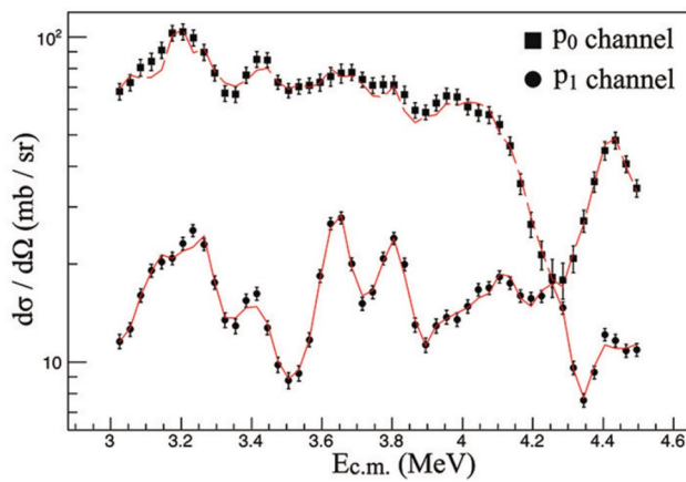
Fig. 8 (Color online) Excitation function for the proton exit channels. p_0 and p_1 represent ^1\text{H}(^{23}\text{Na}, p_0)^{23}\text{Na} and ^1\text{H}(^{23}\text{Na}, p_1)^{23}\text{Na}^*_{440} , respectively
