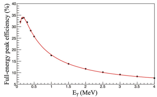
Fig. 3 Efficiency curve of the LaBr 3 array. The black points are the full-energy peak efficiency of the LaBr 3 array for \gamma rays of different energies obtained from Geant4 simulations. The red line represents the fitting result
