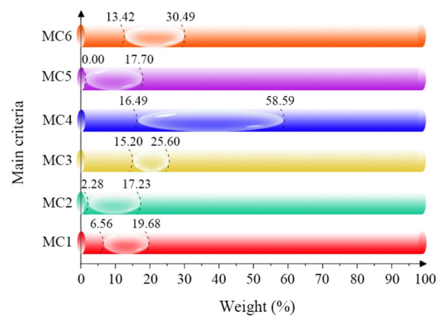
Fig. 11 (Color online) Weight stability interval of MC
