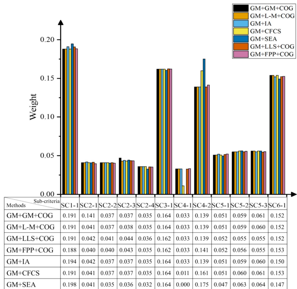
Fig. 5 (Color online) Main- and sub-criteria weights under different methods combinations for fuzzy AHP processes
