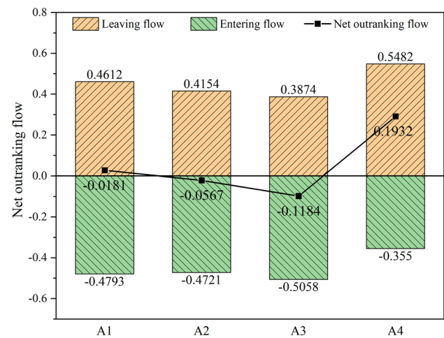
Fig. 7 (Color online) Net ranking flows of four alternatives
