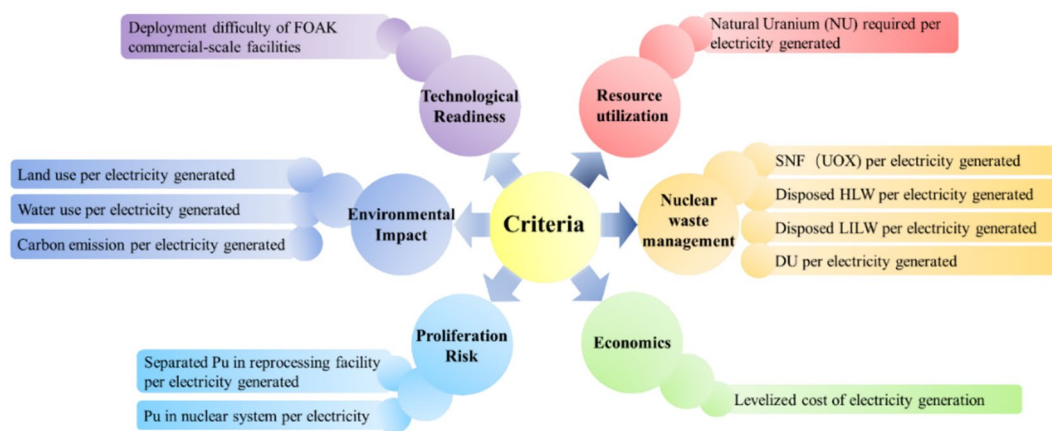
Fig. 3 (Color online) Sustainability-oriented main criteria and sub-criteria
