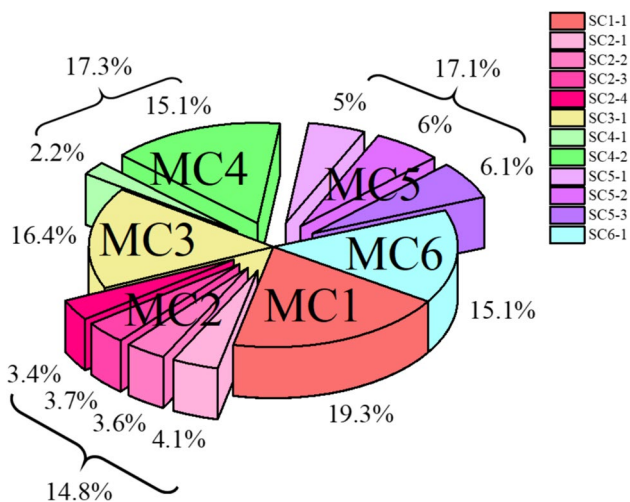
Fig. 6 (Color online) Proportion of the final weights of all criteria
