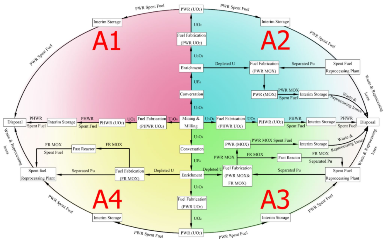
Fig. 2 (Color online) NFC diagram of four candidate alternatives
