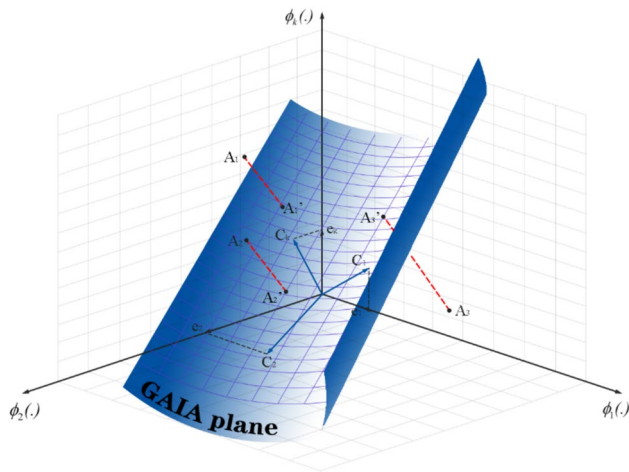
Fig. 4 (Color online) GAIA plane
