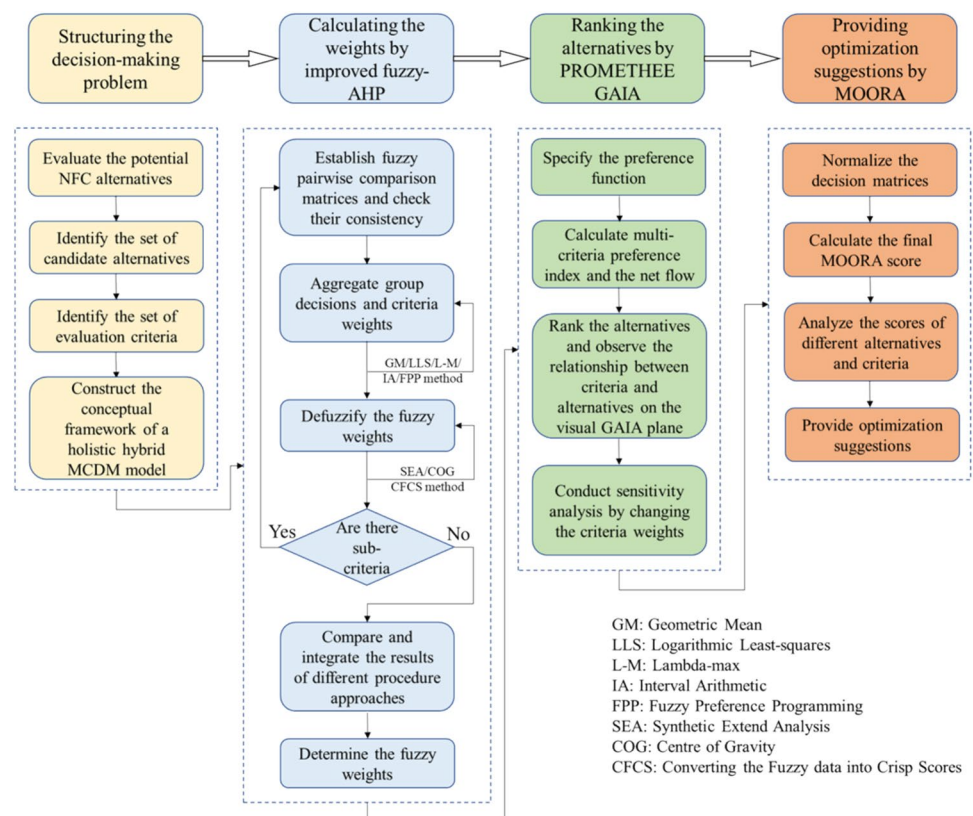
Fig. 1 Overall process diagram of the proposed MCDM framework
