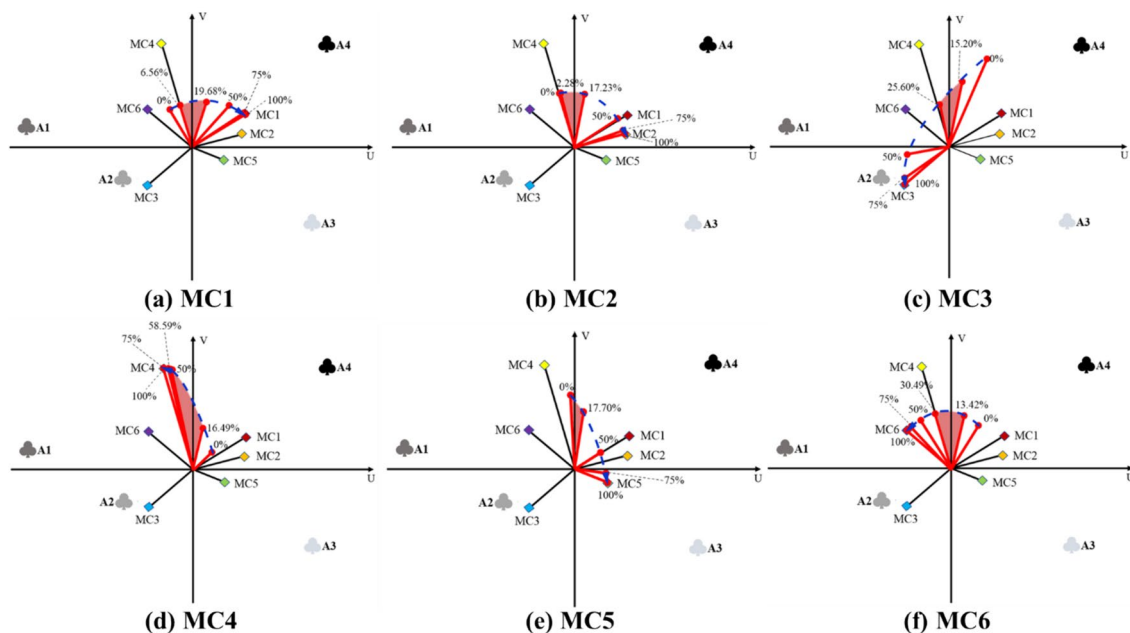
Fig. 10 (Color online) Trajectory of GAIA decision axis in the four alternatives influenced by indicator weights
