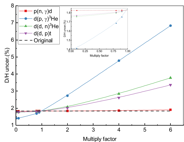
Fig. 1 Calculated D/H uncertainties versus multiplying factor of the reaction-rate uncertainty for the four most important reactions. The connecting lines are used just to guide the eyes. Table 4 can be referenced for details. The inset shows the enlarged plot for the multiplicative factors of M.F. = 0.1, 0.8 and 0.9. Here, the “Original” line (corresponding to a D/H uncertainty of 1.83%) indicates the results calculated with all the default rates and the associated uncertainties adopted in the PRIMAT code [14]
