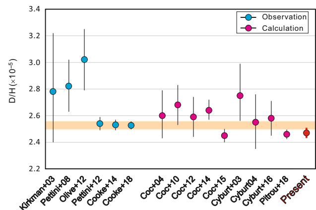
Fig. 2 (Color online) Observational and model calculated primordial deuterium abundances and the associated uncertainties. The data (from left to right) are adopted from Refs. [7, 10–12, 14, 45–53]. The current result shown is calculated by using the recent LUNA d(p,\gamma)^3\text{He} rate, and by considering the uncertainties in \Omega_b h^2 and \tau_n
