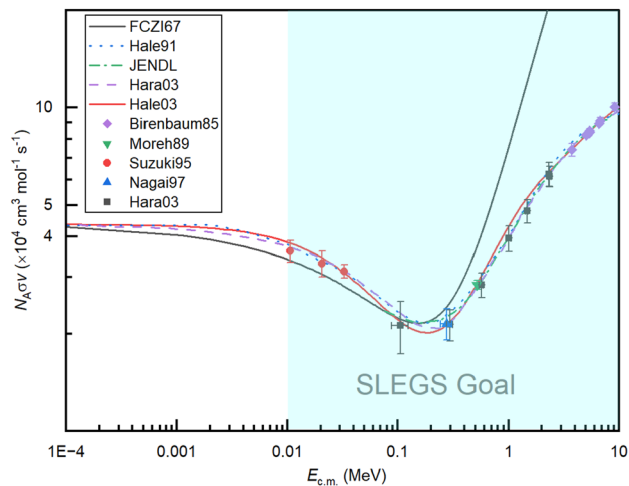
Fig. 3 (Color online) The reaction rate data for p(n,\gamma)d . The black solid line, blue dotted line, red solid line, green dash-dotted line, and purple dashed line are from FCZI [54], Hale in 1991 [55] and in 2003 [56], JENDL [57], and Hara in 2003 [58], respectively. The black square [58], the red circle [59], the blue triangle [60], the green inverted triangle [61] and the purple diamond [62] represent the available experimental data. The shaded area indicates the goal region with the SLEGS facility
