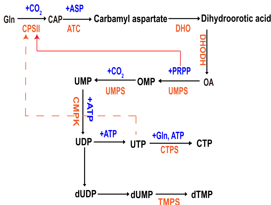
Figure 2 De novo pyrimidine biosynthetic pathway. The first step of pyrimidine synthesis is to produce carbamoyl phosphate. Carbamoyl phosphate synthase II (CPS II) catalyzes the condensation of CO 2 and glutamine. Aspartate carbamoylase (ATCase) catalyzes the condensation of aspartic acid and carbamoyl phosphate to produce carbamoyl aspartate. This reaction is the rate limiting step of pyrimidine synthesis. ATCase is a rate limiting enzyme, which is inhibited by the feedback of the product. It does not consume ATP and is powered by carbamoyl phosphate hydrolysis. Dihydro whey acid with pyrimidine ring was formed by dehydration and intramolecular rearrangement of carbamoyl aspartic acid catalyzed by dihydro whey enzyme. Catalyzed by dihydroorotate reductase, dihydroorotate is oxidized to orotate. This enzyme requires FMN and non heme Fe 2+ , which is located on the outer side of the mitochondrial inner membrane. Quinones provide oxidation ability. The other five enzymes in pyrimidine synthesis exist in the cytosol. The reaction of whey acid with PRPP was catalyzed by whey acid phosphoribosyltransferase to produce orotidine-5'-monophosphate (OMP). It is powered by PRPP hydrolysis. OMP decarboxylase catalyzes OMP decarboxylation to produce UMP. The synthesis of uridine triphosphate (UTP) is similar to that of purine nucleoside triphosphate. Cytidine triphosphate (CTP) is produced by ammonia addition of UTP catalyzed by CTP synthase. In animals, the amino group is provided by glutamine, while in bacteria, it is directly provided by NH 3 . This reaction consumes 1 ATP.
