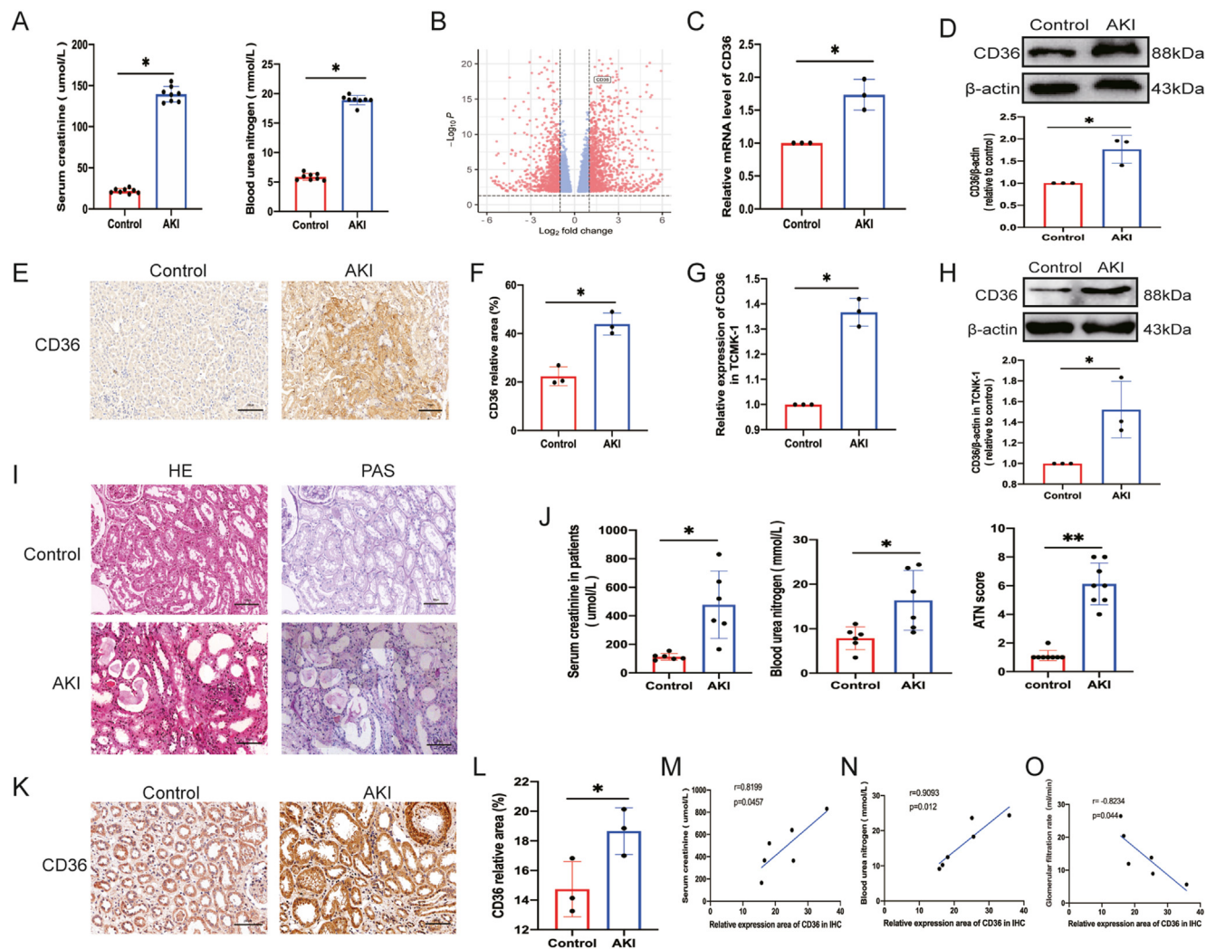
Figure 1 CD36 expression level was increased in AKI. (A) Cisplatin-induced AKI with elevated Scr and BUN levels ( n = 8 ; * P < 0.05 vs. control group). (B) Transcriptome sequencing results indicated that CD36 gene was up-regulated. (C) CD36 mRNA level in mouse kidney ( n = 3 ) quantified via qPCR. (D) Western blotting was used to detect CD36 expression in mouse kidney tissues ( n = 3 ). (E) Representative images of immunohistochemical staining and quantitative statistics of relative CD36 area in mice ( n = 3 ). (F) Quantitative statistical analysis of relative CD36 area from (E). (G) CD36 mRNA level in TCMK-1 cells ( n = 3 ) quantified via qPCR. (H) Western blotting was used to detect CD36 expression in TCMK-1 cells ( n = 3 ). All data are expressed as means ± standard deviation. * P < 0.05 and ** P < 0.01 vs. control group. (I) Representative CD36 images of immunohistochemical and pathological sections (HE and PAS) in kidney tissue samples from clinical patients. Scale bars = 100 μm. (J) Renal function levels, including Scr, BUN, and GFR in clinical samples. (K) Representative immunohistochemical staining images of relative CD36 area in human AKI sample. (L) Quantitative statistical analysis of relative CD36 area from (K). (M–O) Pearson correlation analysis between CD36 expression and renal function.
