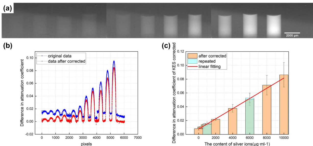
Fig. 3 (Color online) Consistency evaluation of different experiments. a KES images of Ag arranged in an ascending order of concentration for the three phantoms. b Original grayscale of KES
