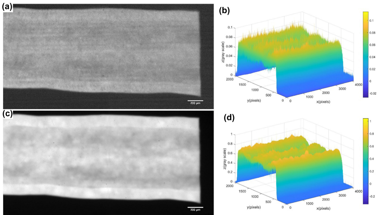
Fig. 4 (Color online) KES imaging of lead-free solder. a KES image of element Ag in lead-free solder. b Surface plot of the grayscale of the image shown in a . c Absorption image of lead-free solder at 25.43 keV. d The corresponding grayscale of the image shown in c
