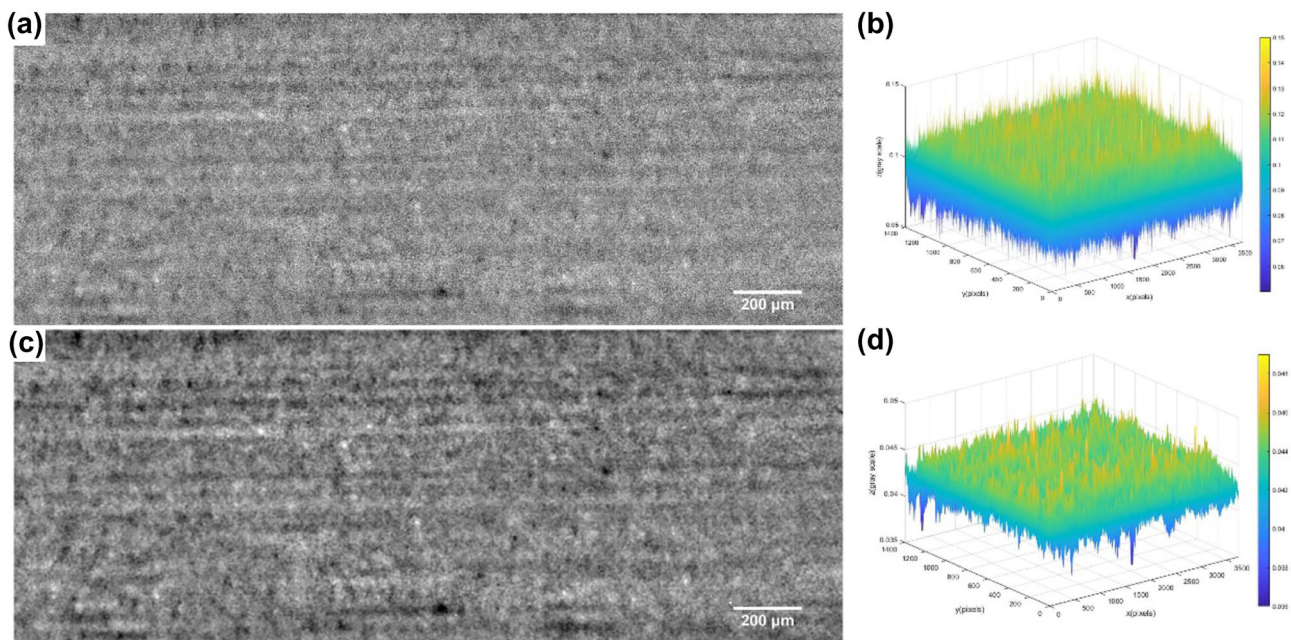
Fig. 5 (Color online) Distribution characteristics of element Ag in the alloy sheet with normalized sample thickness. a KES image with noises. b Surface plot of the concentration distribution of the element
