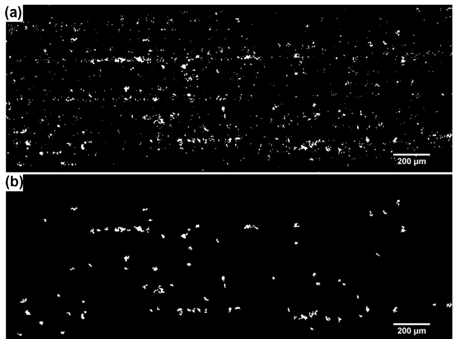
Fig. 5 (Color online) Distribution characteristics of element Ag in the alloy sheet with normalized sample thickness. a KES image with noises. b Surface plot of the concentration distribution of the element
