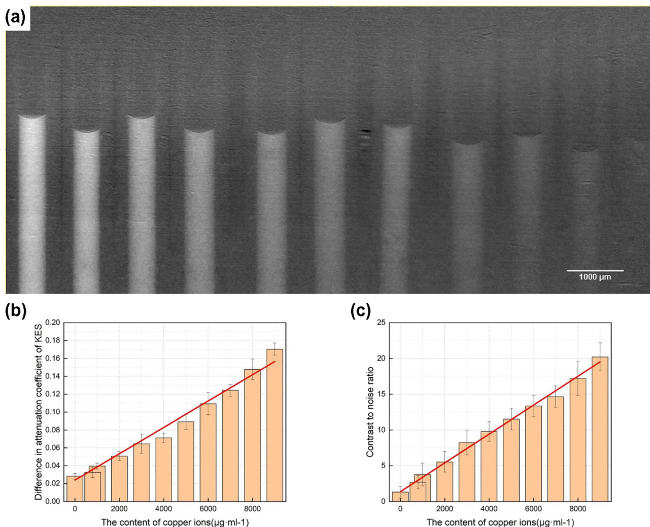
Fig. 2 (Color online) Cu content in a KES image: a element distribution in the eleven sample tubes, b grayscale distribution after attenuation by samples with different concentrations of Cu element, and c calibrated grayscale according to contrast to noise ratio of the KES image
