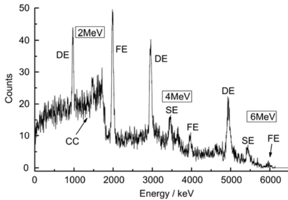
Fig.3 Simulated spectrum for single crystal output in BGO array (CC: Compton-Continuous Spectrum, SE: Single-Escape Peak, DE: Double-Escape Peak, and FE: Full-Energy Peak).
