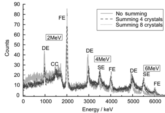
Fig.5 Spectrums with and without the correction.
