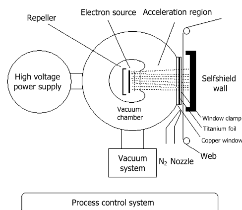
Fig.1 Electron curtain accelerator diagram.
