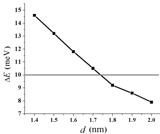
Fig. 3. Convergence test of the vacuum thickness for the UN(001) surface.
