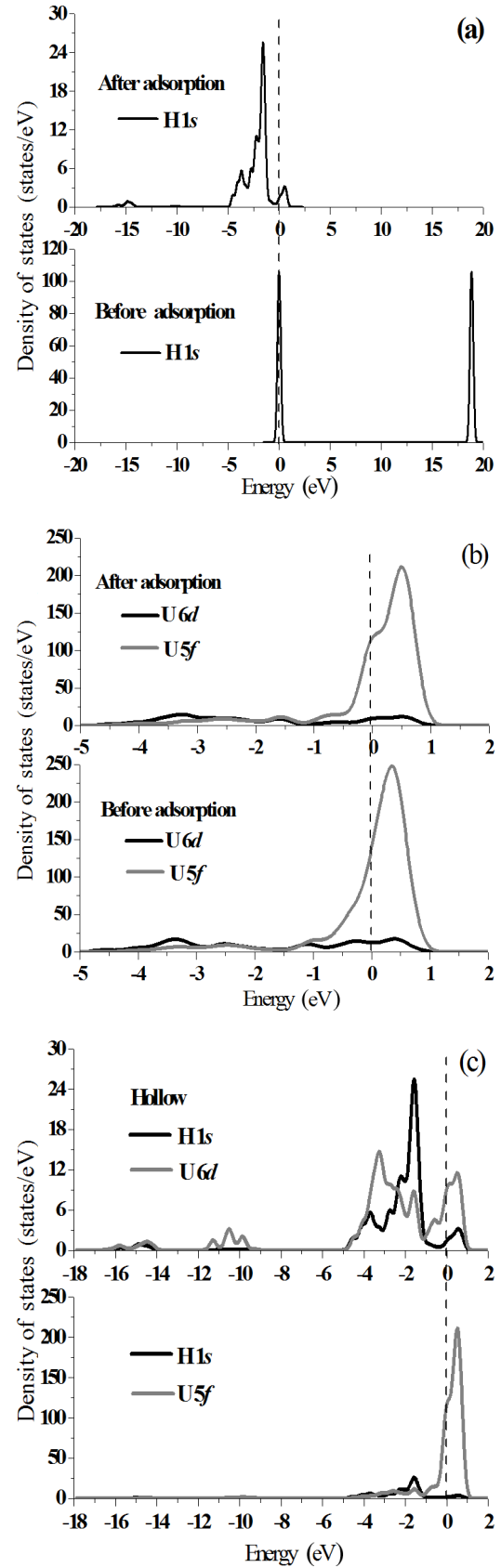
Fig. 5. Projected density of states (PDOS) of H 1s orbital (a), U 6d, 5f orbitals (b) and H 1s, U 6d, 5f orbitals (c) before and after H chemisorption on the Hollow position of UN(001) surface. The Fermi energy (dash line) stands at 0 eV.
