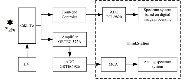
Fig. 6. The block diagram of the experimental apparatus.
