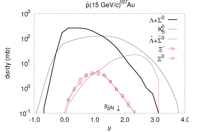
Fig. 9. (Color online) The rapidity spectra of (\Lambda + \Sigma^0) , K_S^0 , (\bar{\Lambda} + \bar{\Sigma}^0) , \Xi^- , and \Xi^0 from \bar{p}^{197}\text{Au} collisions at 15 GeV/c.
