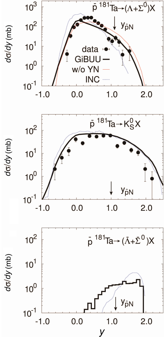
Fig. 7. (Color online) Rapidity spectra of (\Lambda + \Sigma^0) , K_S^0 , and (\bar{\Lambda} + \bar{\Sigma}^0) from \bar{p}^{181}\text{Ta} collisions at 4 GeV/c. See text for details.
