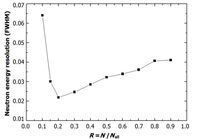
Fig. 4. Neutron energy resolution vs. number of fitting track points.
