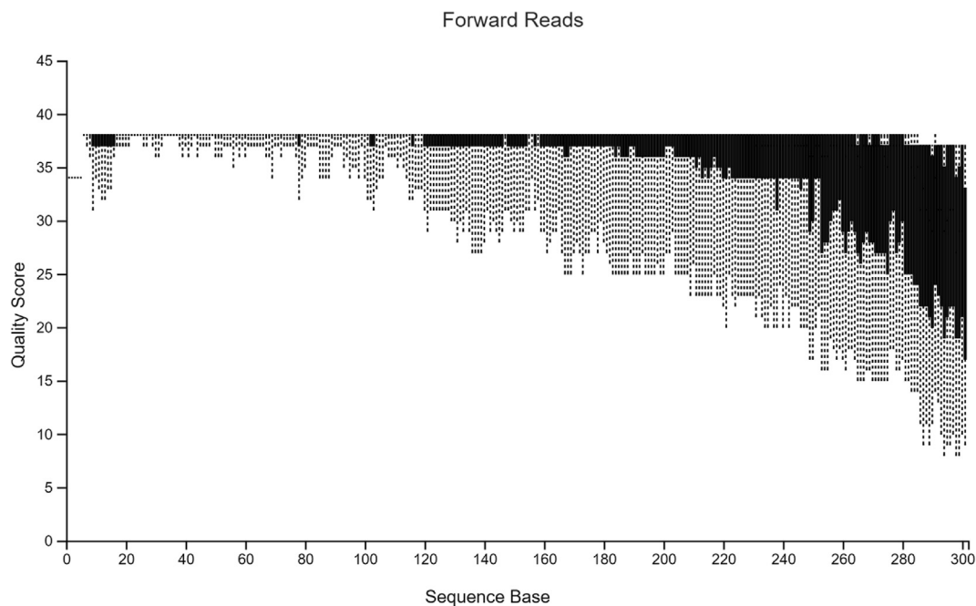
Figure 6 Quality plot for Forward Reads for the Second Pre-clinical data.
