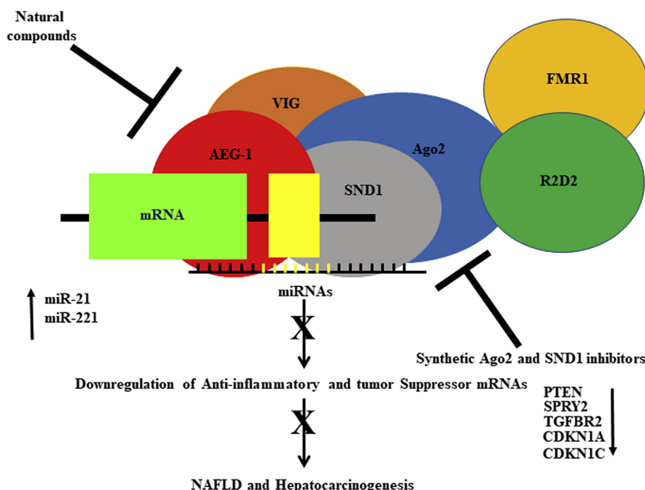
Figure 2 The possible mechanism of RNA-induced silencing complex and its components as novel targets for Hepatocellular Carcinoma therapy.
