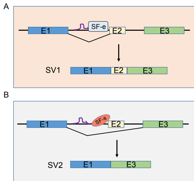
Fig. 1 A simplified model for lncRNA-mediated alternative splicing. A , lncRNA promotes inclusion of Exon2 (E2) by interaction with enhancing splicing factor (SF-e) to form splice variant 1 (SV-1). B , lncRNA promotes skipping of Exon2 (E2) by interaction with silencing splicing factor (SF-s) to form splice variant 2 (SV-2).
