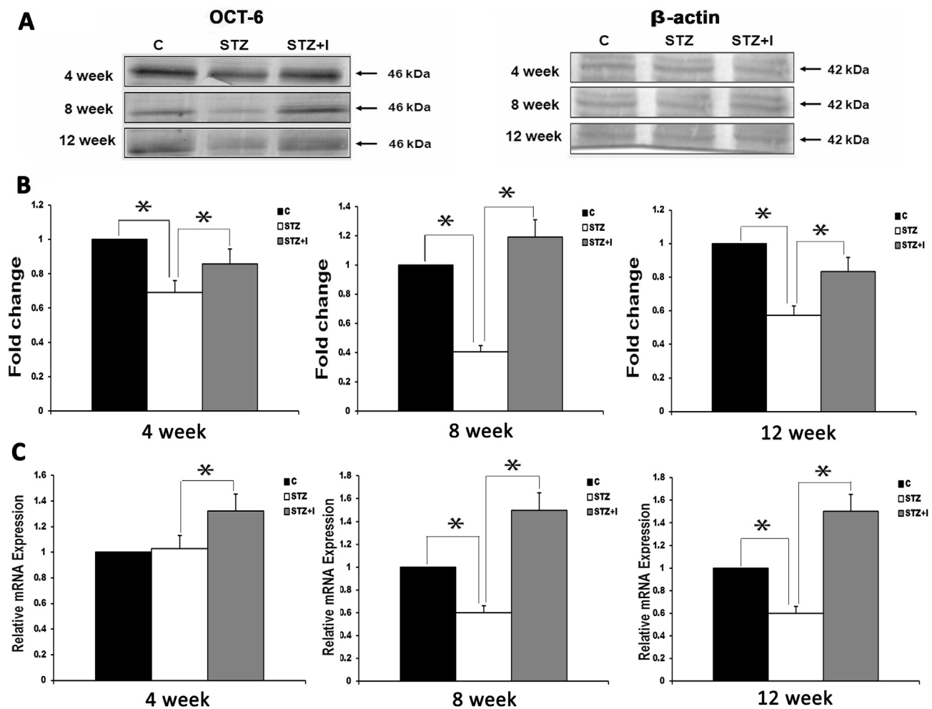
Figure 2 Differential expression of OCT-6 protein and OCT-6 mRNA level at 4, 8 and 12 week sciatic nerve samples correlated between control (C), diabetic (STZ) and insulin treated diabetic rats (STZ+I). (A) Western blot analysis for OCT-6 protein expression of sciatic nerve in STZ and STZ+I compared to Control. \beta actin was used for normalization. (B) Western blotting data were presented as a bar chart. (C) Real time PCR studies showing change in relative mRNA expression of OCT-6 among STZ and STZ+I of sciatic nerve. RPL19 was used as house keeping gene.*indicates p < 0.05 .
