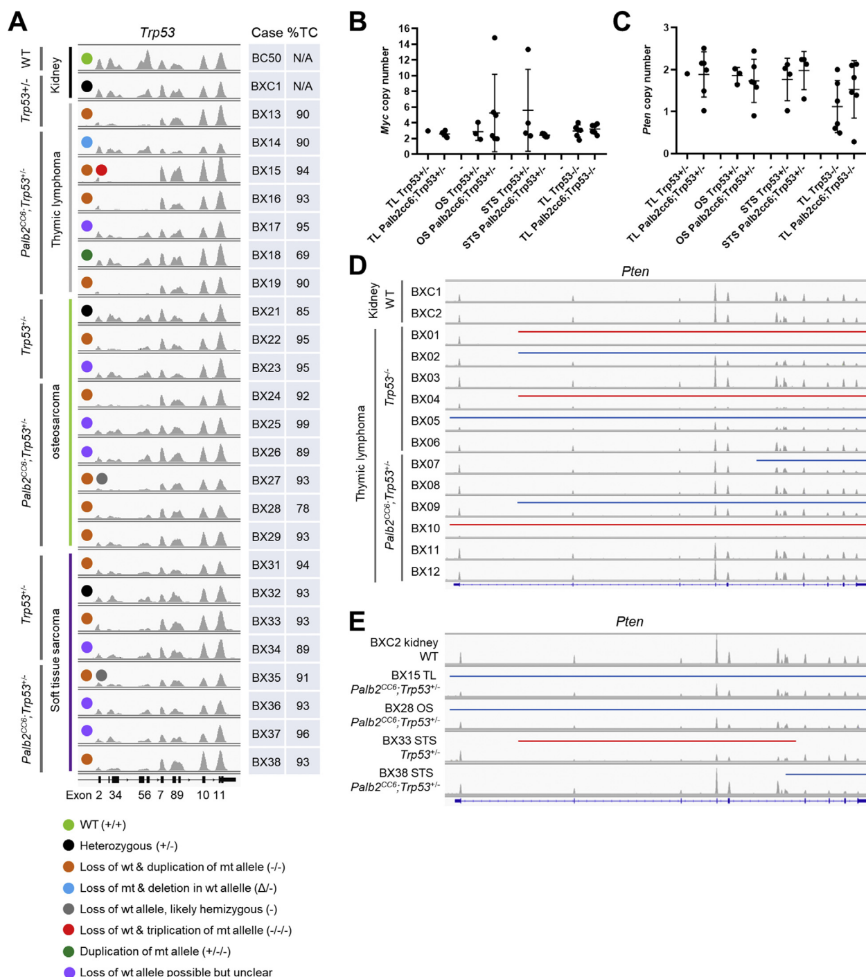
Figure 2 Genomic analyses of tumors from Palb2 CC6 mutant mice in different Trp53 backgrounds. (A) Status of the Trp53 locus in tumors from Trp53 +/- and Palb2 CC6 ;Trp53 +/- mice. Images were generated with IGV based on WES data. Data range for each track is normalized using the size of the corresponding BAM file, which reflects the number of total reads obtained for the tumor. (B,C) Dot plots of computed copy numbers of Myc (B) and Pten (C) in all tumors sequenced. (D,E) Status of the Pten locus in all 12 sequenced tumors from Trp53 -/- and Palb2 CC6 ;Trp53 +/- mice (D) and selected tumors from Palb2 CC6 ;Trp53 +/- mice (E). Data range for each track is normalized as in A. Regions of monoallelic and biallelic deletion are indicated by blue and red bars, respectively.
