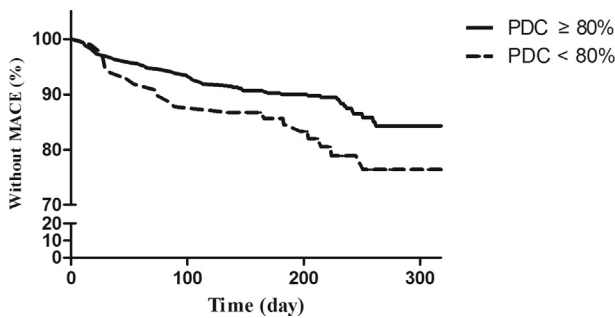
Figure 2 The survival curves for people with PDC \geq 80\% and with PDC < 80\% . The solid line stands for the percentage of PDC \geq 80\% patients without end points over time, while the dotted line stands for the percentage of PDC < 80\% patients without end points over time. Patients with PDC \geq 80\% were significantly longer-lived than those with PDC < 80\% ( p < 0.05 ). Abbreviations: PDC, proportion of days covered; MACE, major adverse cardiac events.
