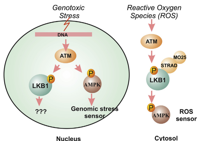
Figure 3 The role of LKB1 as a ROS sensor but not a genomic stress sensor. Ionization radiation activates ATM and AMPK in a LKB1-independent manner to sense genomic stress. LKB1/AMPK is required for reactive oxygen species (ROS) to activate mTOR through cytosolic ATM.
