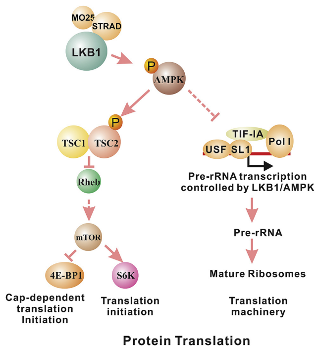
Figure 2 AMPK regulates protein translation through its effects on mTOR and pre-rRNA synthesis. The activation of AMPK suppresses mTOR activity, thus interfering with translation initiation. AMPK also phosphorylates TIF-IA to prevent the assembly of pre-rRNA transcription initiation complex, thus prevent the synthesis of ribosome which is required for protein translation.
