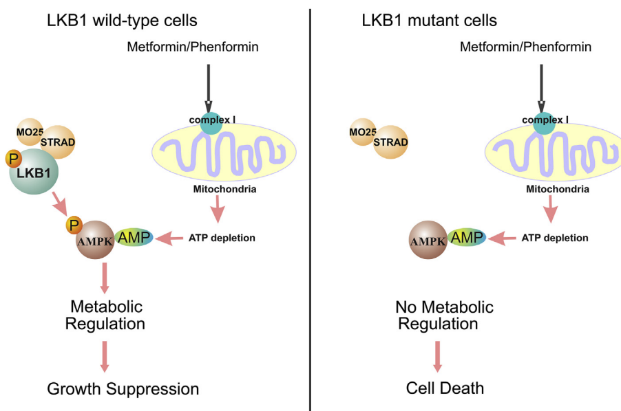
Figure 1 The effects of AMPK activators in LKB1-wild type and mutant cells. Metformin and phenformin inhibit mitochondria complex I, which results in the depletion of intracellular ATP and increases in AMP. The binding of AMP to the AMPK activates AMPK kinase activity and its metabolic regulation function. The lack of LKB1 prevents the activation of AMPK by AMP. As a result, metformin and phenformin induced energetic stress cannot be properly detected in LKB1-mutant cells, which eventually lead to cell death.
