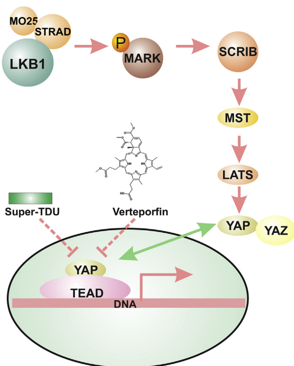
Figure 4 LKB1 negatively regulates YAP1 function. LKB1 regulates SCRIB cellular localization through its phosphorylation of MARK. The proper cellular localization of SCRIB is required for the regulation of YAP phosphorylation by its upstream kinases, such as MST and LATS.
