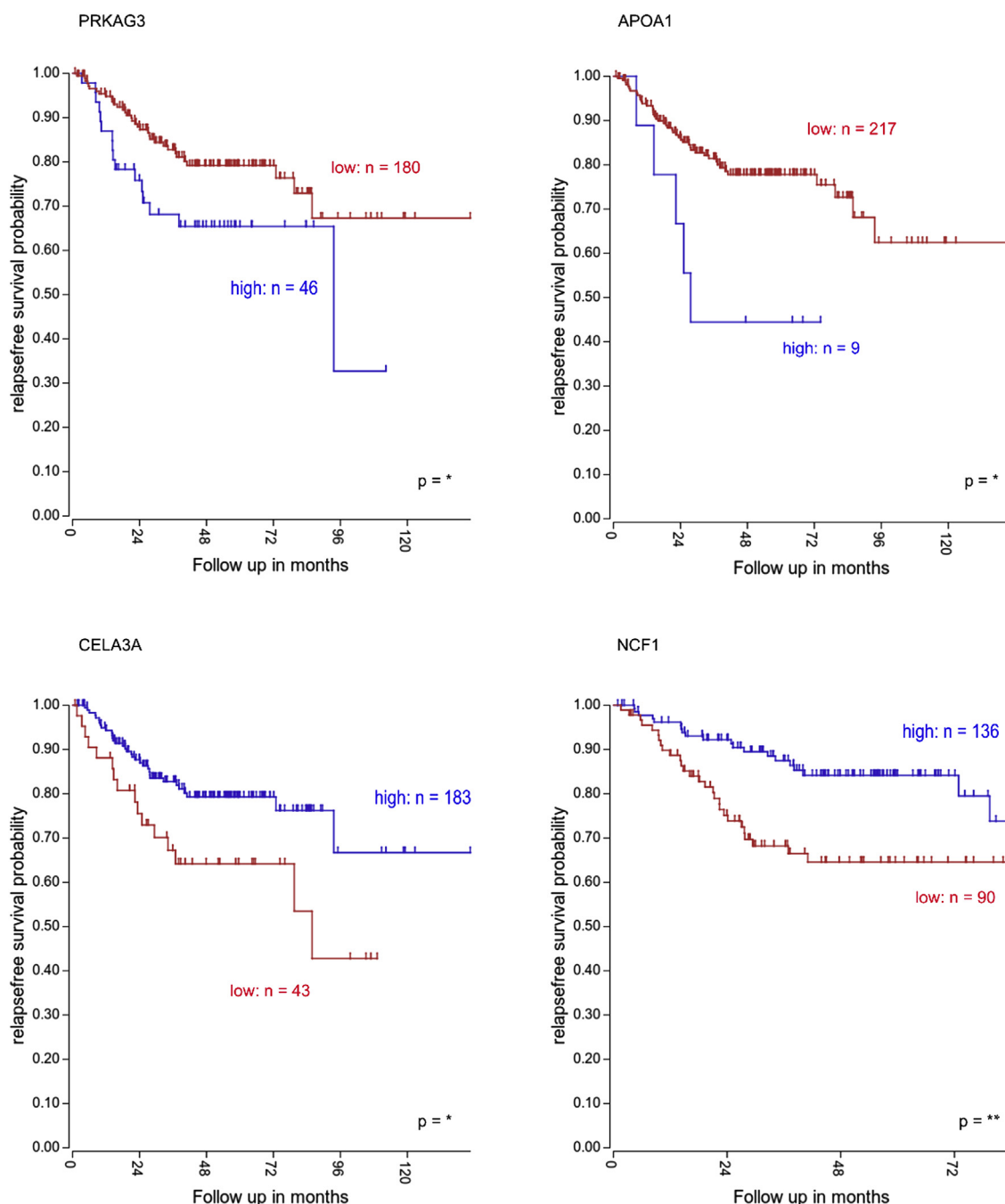
Figure 7 Clinical impact of genes involved in lipid metabolism and oxidative stress. Relapse-free survival (RFS) rate of CRC patients (Tumor Colon-Siebert database) according to PRKAG3, APOA1, CELA3A and NCF1 expression levels.
