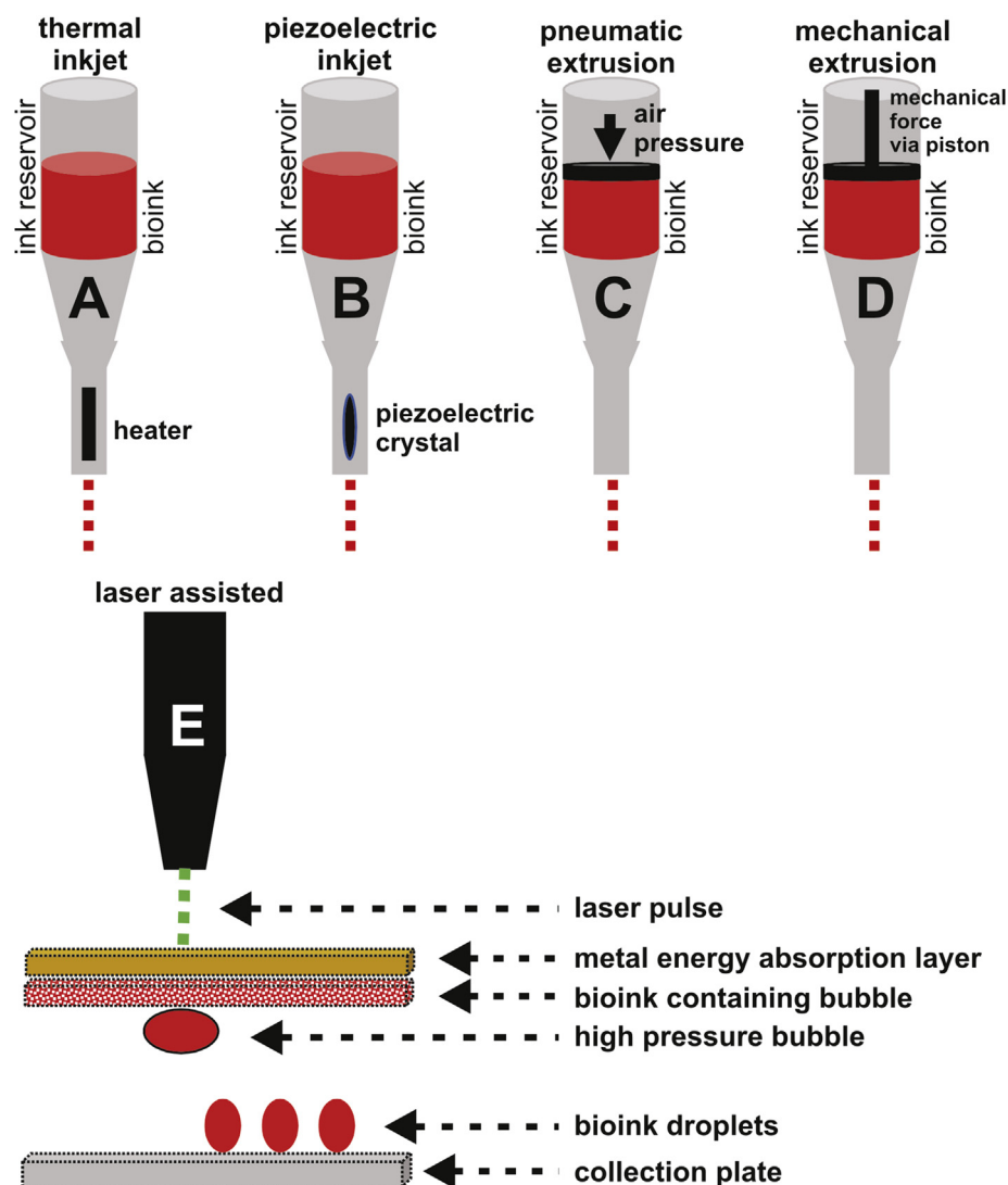
Figure 2 Schematic depicting the most common bioprinting methods. (A) Thermal Inkjet Bioprinting. (B) Piezoelectric Inkjet Bioprinting. (C) Pneumatic Extrusion Bioprinting. (D) Mechanical Extrusion Bioprinting. (E) Laser-Assisted Bioprinting.
